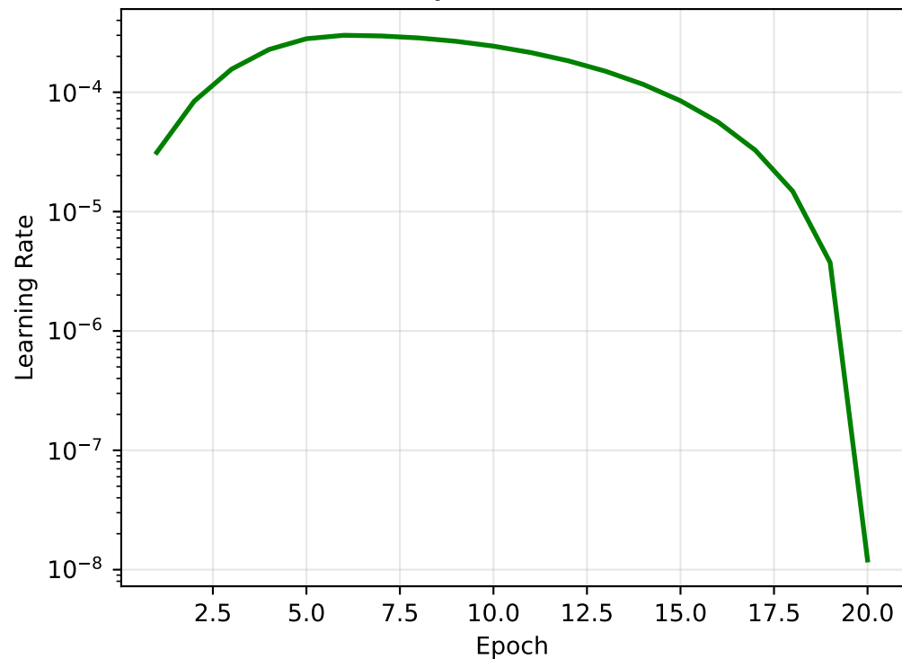
OneCycleLR Schedule
